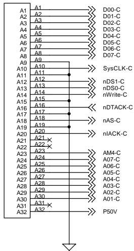
XP10A Harting-41612-96
