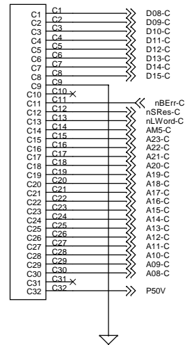
XP10C Harting-41612-96
