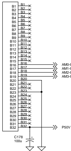
XP10B Harting-41612-96
