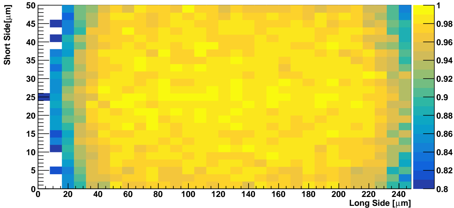
Efficiency Pixel Map DUT 22 Geometry 0
