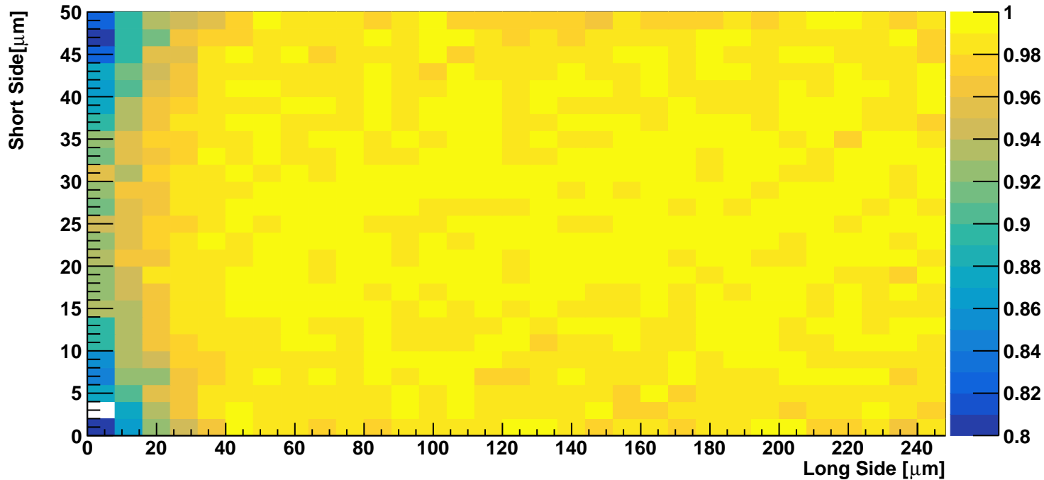
Efficiency Pixel Map DUT 21 Geometry 0
