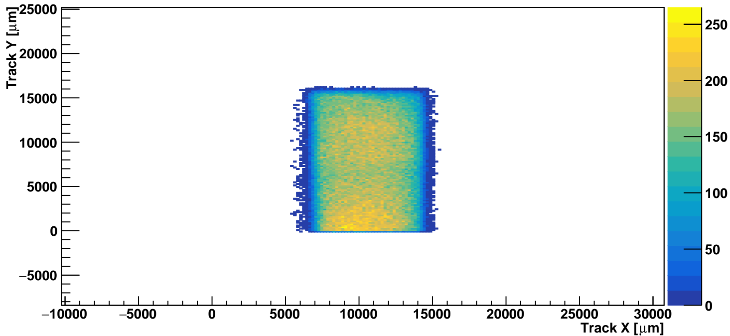
Beam profile DUT 22
