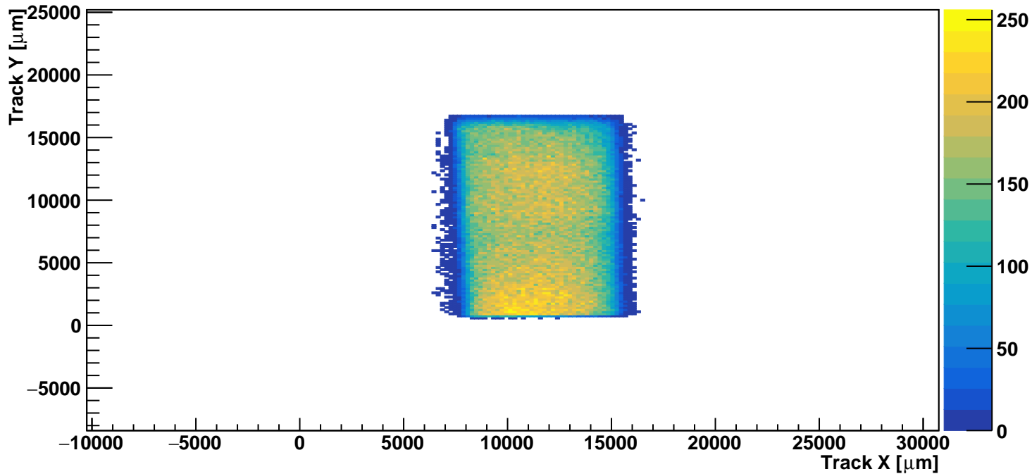
Beam profile DUT 21
