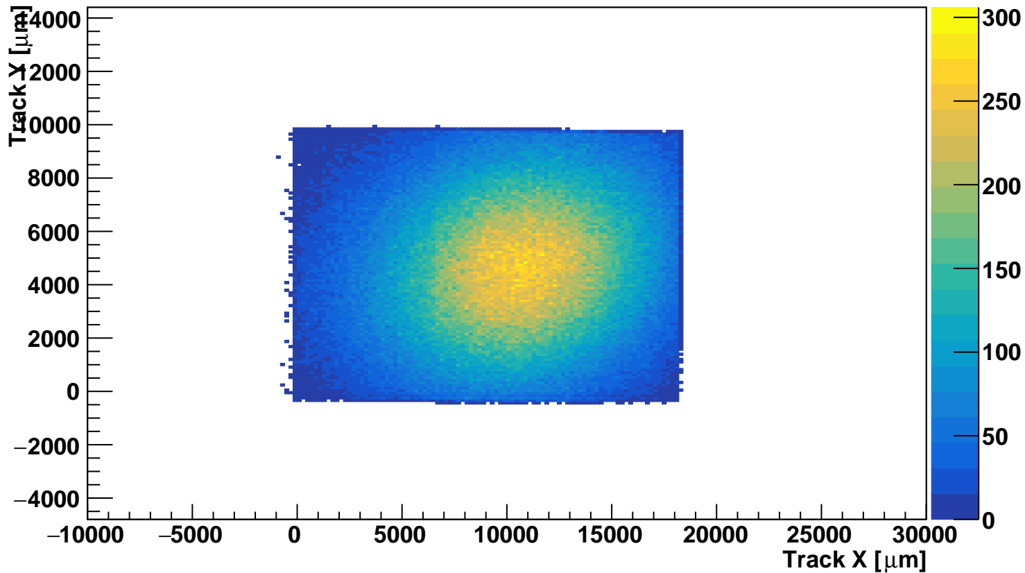
Beam profile no angle cut DUT 30
