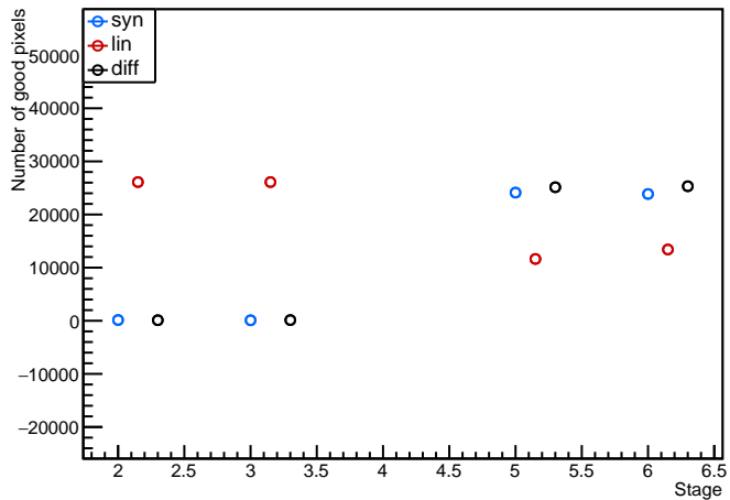
Module: Paris21, 20UPGFC0013659 (FE2) discbumpscan Evolution plot (98<occupancy<102)
