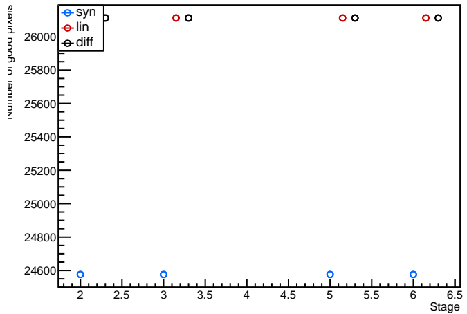
Module: Paris21, 20UPGFC0013404 (FE3) digitalscan Evolution plot (97<occupancy<103)
