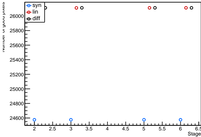
Module: Paris21, 20UPGFC0013659 (FE2) digitalscan Evolution plot (97<occupancy<103)
