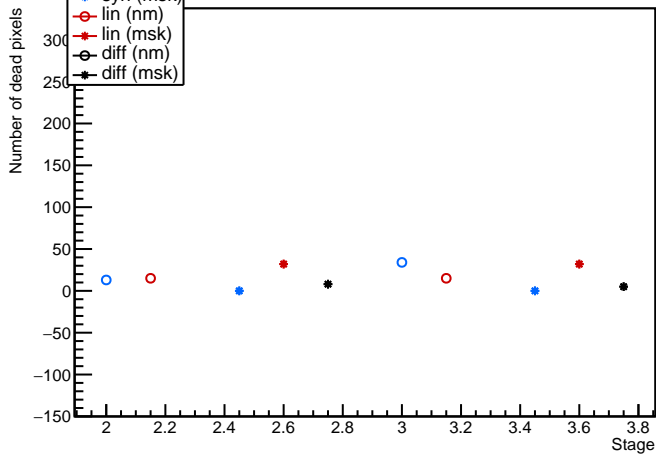
Module: MilanQ5, 20UPGFC0013401 (FE2) discbumpscan Evolution plot (occupancy=0)
