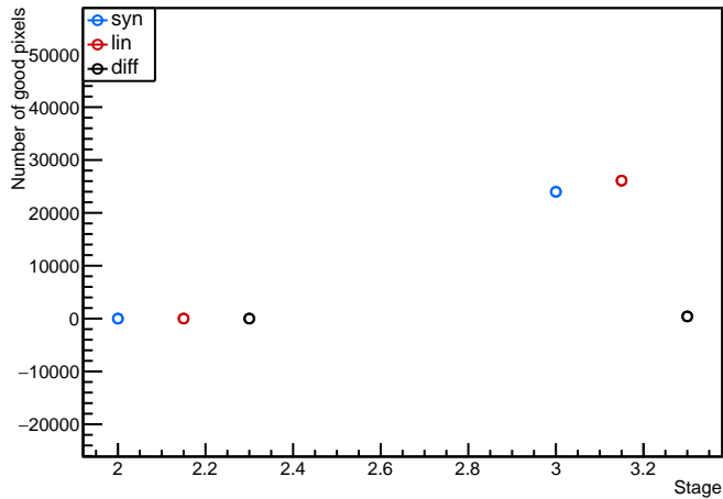
Module: MilanQ5, 20UPGFC0013434 (FE3) discbumpscan Evolution plot (98<occupancy<102)
