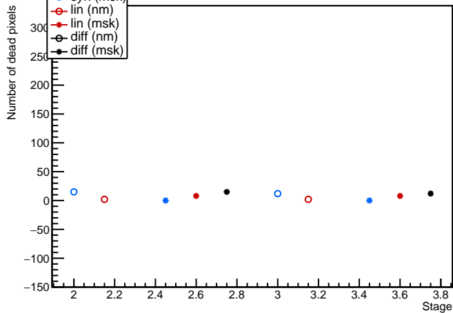
Module: MilanQ5, 20UPGFC0013434 (FE3) discbumpscan Evolution plot (occupancy=0)
