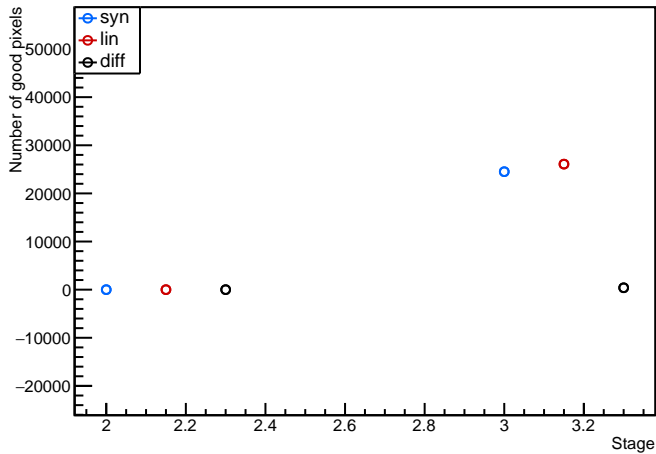
Module: MilanQ5, 20UPGFC0013461 (FE1) discbumpscan Evolution plot (98<occupancy<102)
