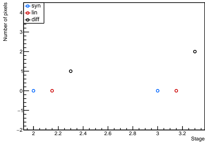
Module: MilanQ5, 20UPGFC0013401 (FE2) analogscan Evolution plot (occupancy>102)
