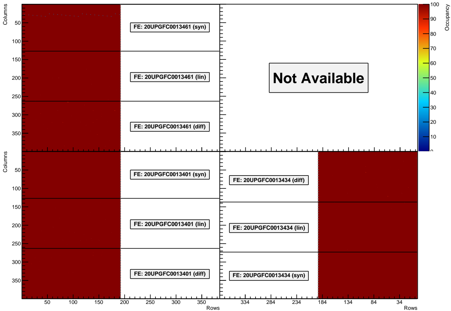
analogscan OccupancyMap (Module: MilanQ5) (Stage3)
