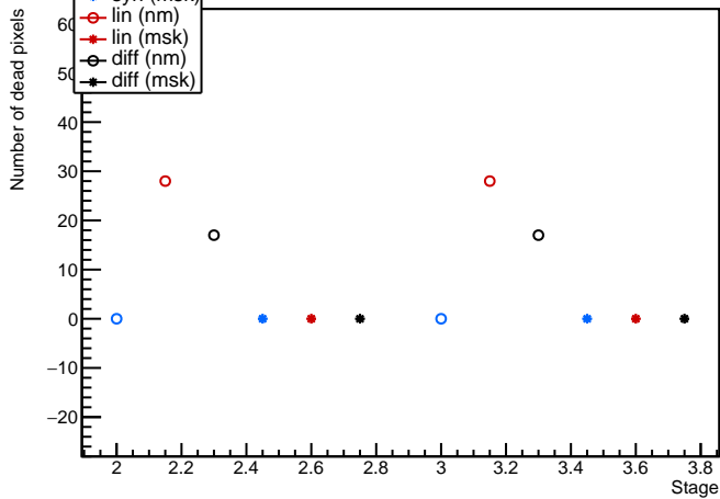
Module: MilanQ5, 20UPGFC0013461 (FE1) analogscan Evolution plot (occupancy=0)
