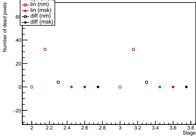
Module: MilanQ5, 20UPGFC0013401 (FE2) analogscan Evolution plot (occupancy=0)
