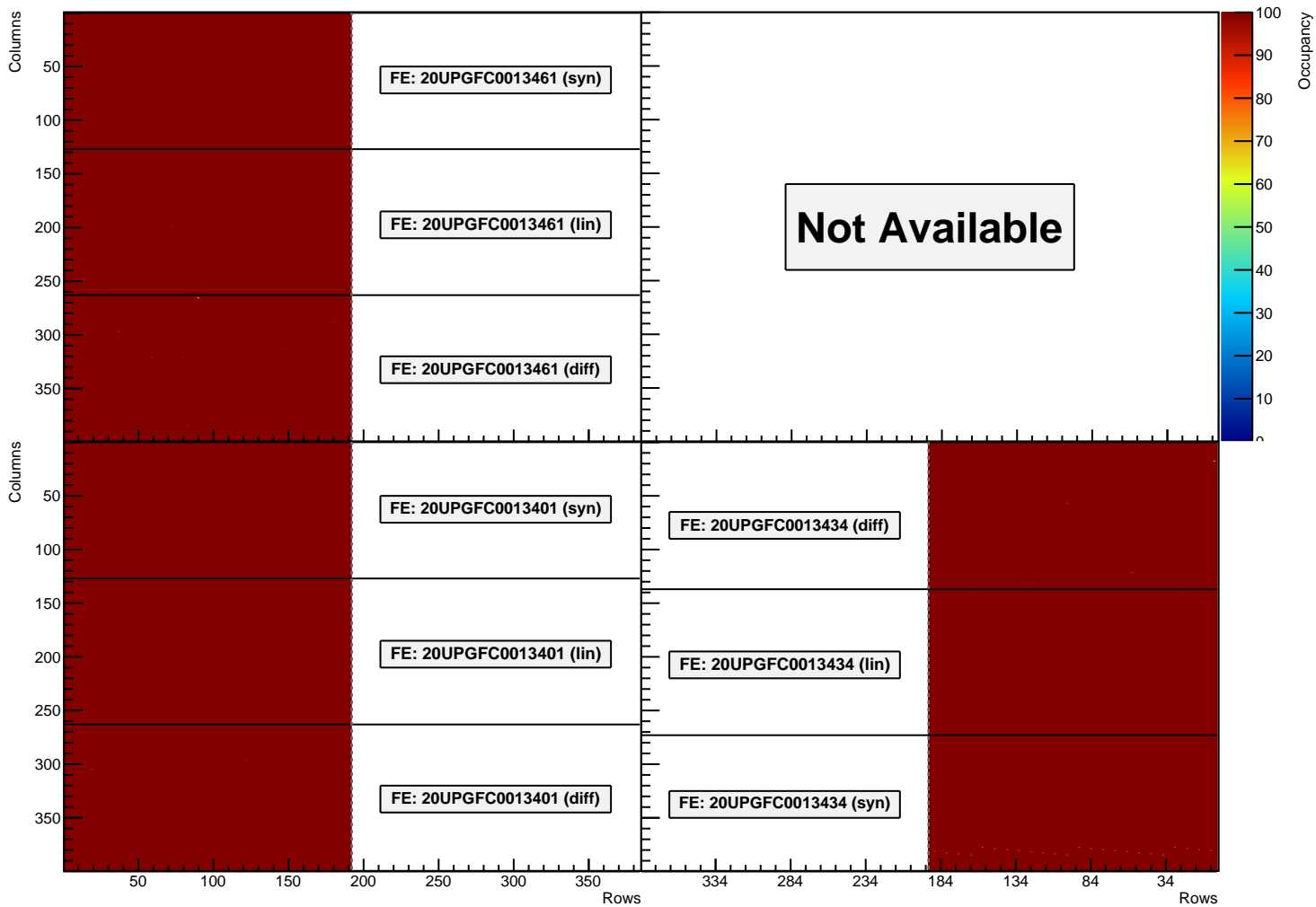
analogscan OccupancyMap (Module: MilanQ5) (Stage2)
