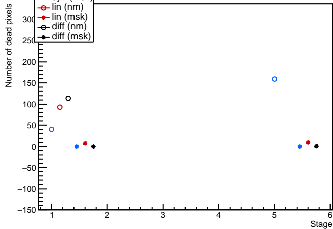
Module: MilanQ3, 20UPGFC0012872 (FE2) discbumpscan Evolution plot (occupancy=0)
