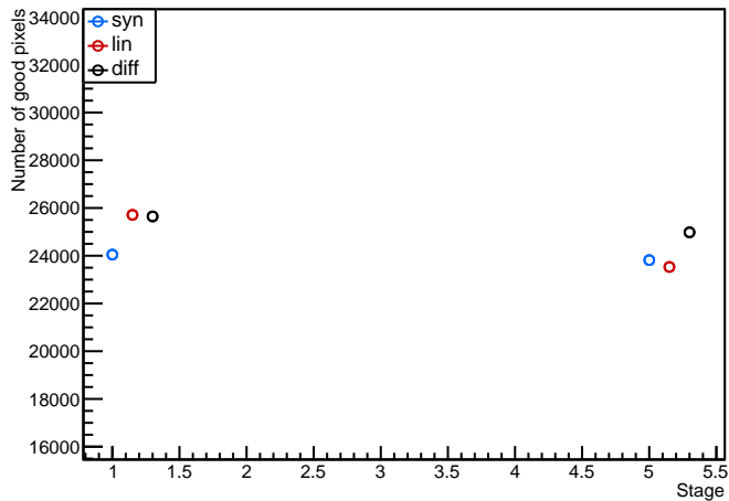
Module: MilanQ3, 20UPGFC0009290 (FE3) discbumpscan Evolution plot (98<occupancy<102)
