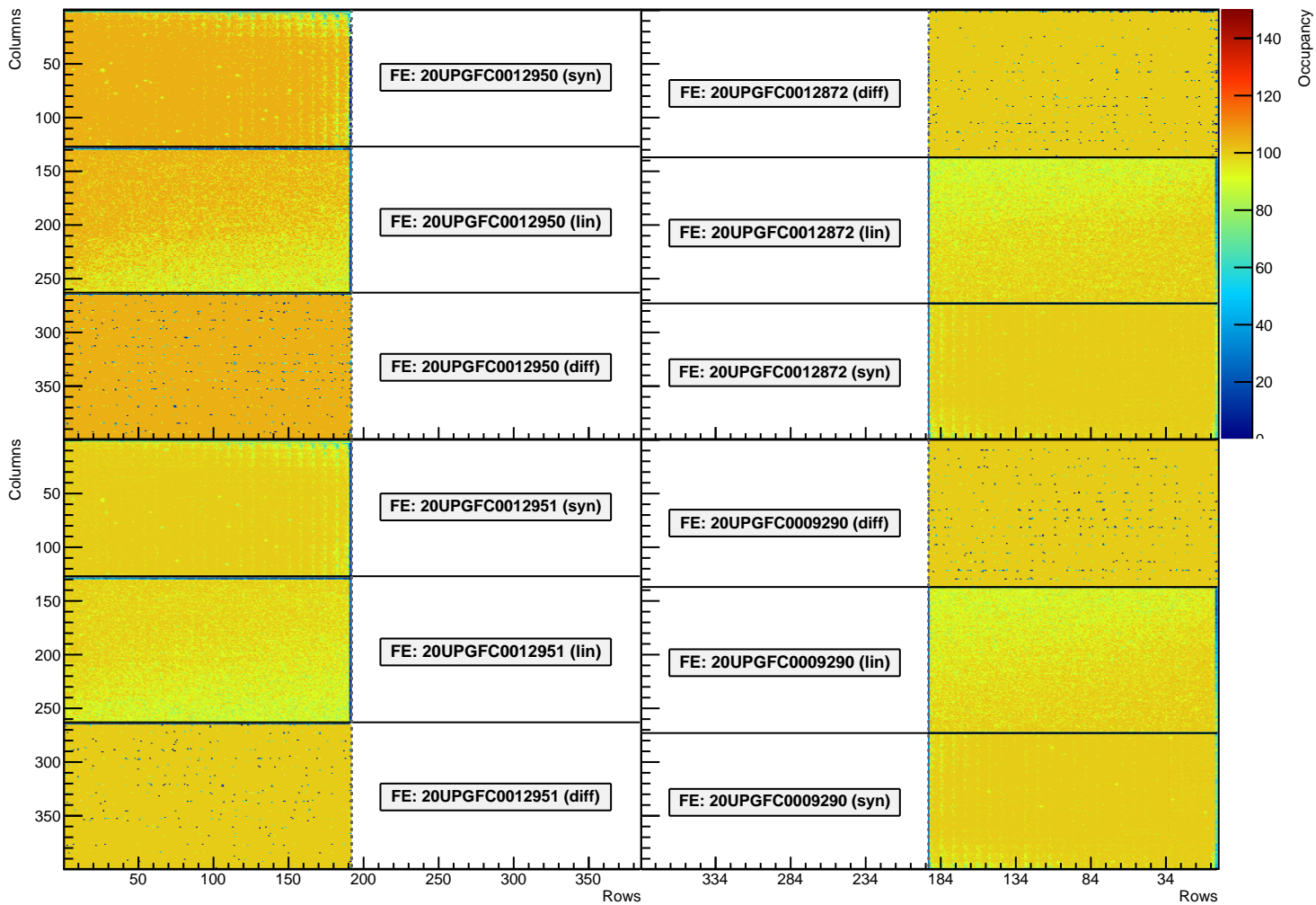
discbumpscan OccupancyMap (Module: MilanQ3) (Stage4)
