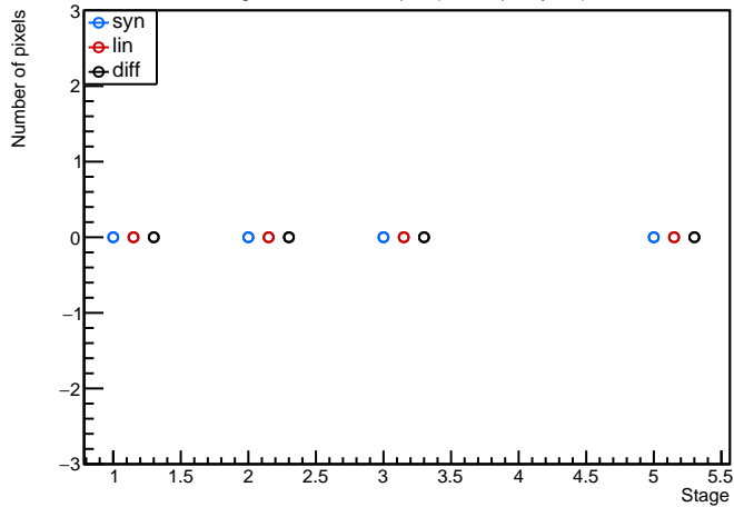
Module: MilanQ3, 20UPGFC0012951 (FE2) digitalscan Evolution plot (0<occupancy<98)
