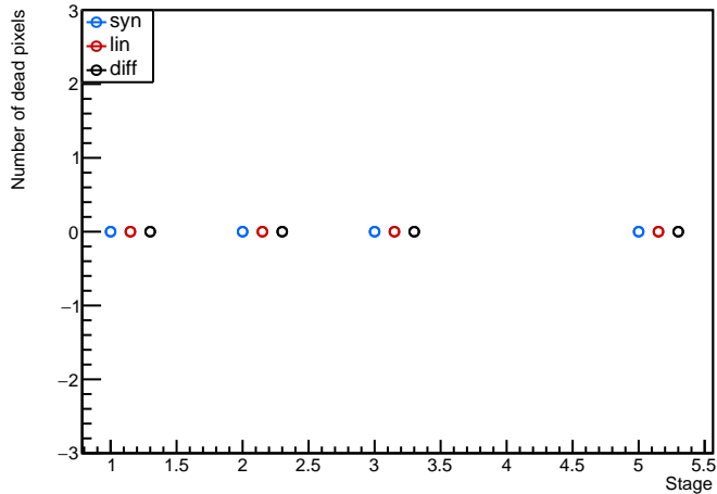
Module: MilanQ3, 20UPGFC0012951 (FE2) digitalscan Evolution plot (occupancy=0)
