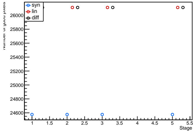
Module: MilanQ3, 20UPGFC0009290 (FE3) digitalscan Evolution plot (97<occupancy<103)
