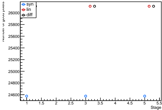
Module: MilanQ2, 20UPGFC0008777 (FE4) digitalscan Evolution plot (97<occupancy<103)
