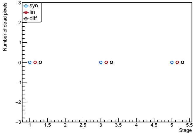
Module: MilanQ2, 20UPGFC0008777 (FE4) digitalscan Evolution plot (occupancy=0)
