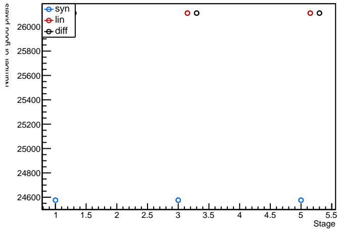
Module: MilanQ2, 20UPGFC0008794 (FE3) digitalscan Evolution plot (97<occupancy<103)
