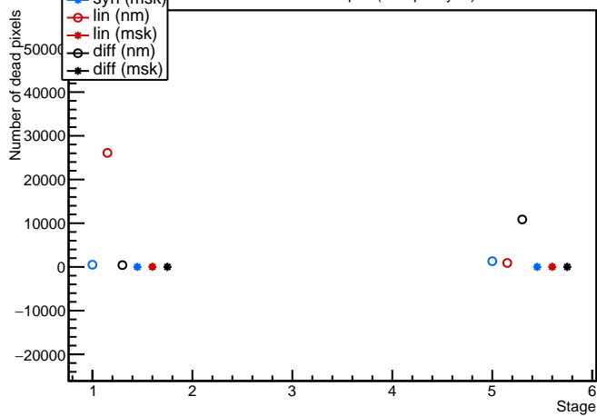
Module: MilanQ2, 20UPGFC0008794 (FE3) crosstalkscan Evolution plot (occupancy=0)
