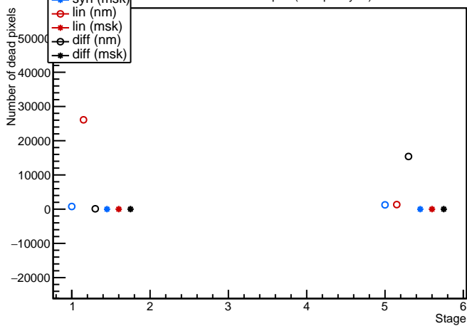
Module: MilanQ2, 20UPGFC0012412 (FE2) crosstalkscan Evolution plot (occupancy=0)
