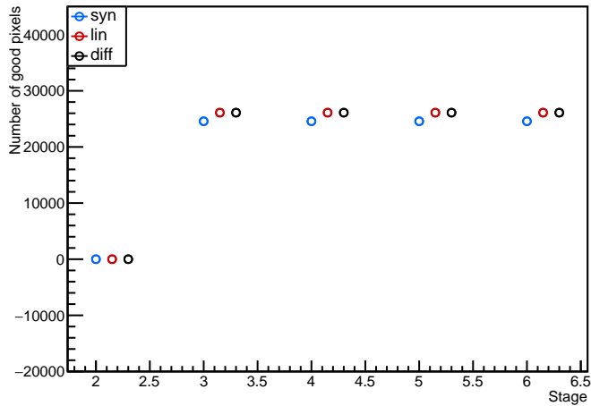
Module: LivThn6, 20UPGFC0012935 (FE3) digitalscan Evolution plot (97<occupancy<103)
