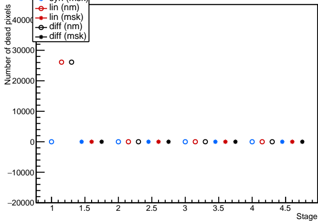
Module: LivThn6, 20UPGFC0012856 (FE2) analogscan Evolution plot (occupancy=0)
