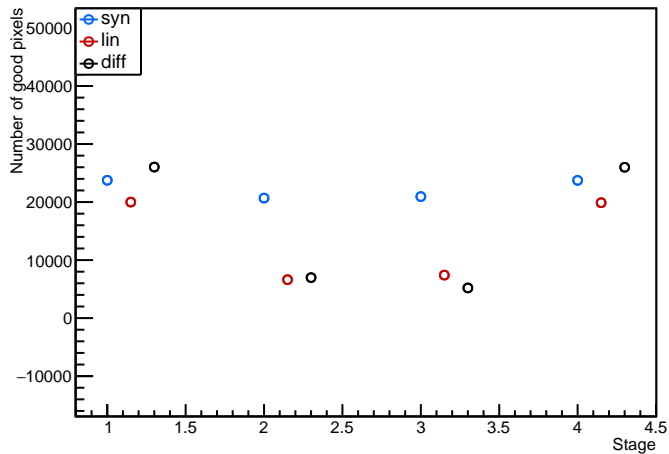
Module: LivThn1, 20UPGFC0009306 (FE2) discbumpscan Evolution plot (98<occupancy<102)
