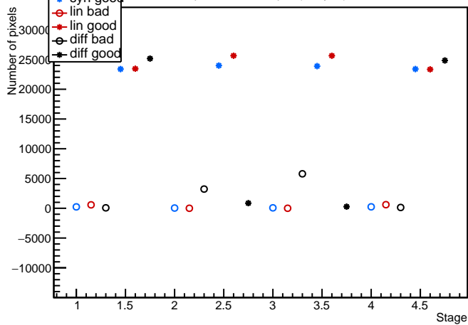
Module: LivThn1, 20UPGFC009322 (FE3) discbumpscan Evolution plot (analysis)
