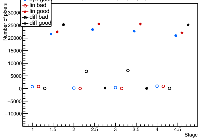
Module: LivThn1, 20UPGFC009370 (FE4) discbumpscan Evolution plot (analysis)
