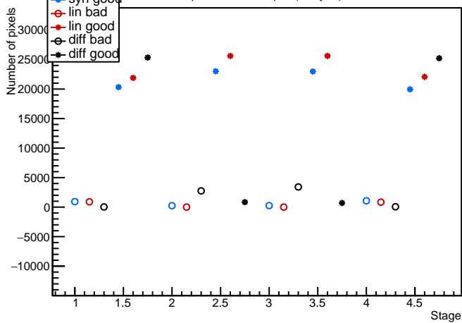
Module: LivThn1, 20UPGFC009274 (FE1) discbumpscan Evolution plot (analysis)
