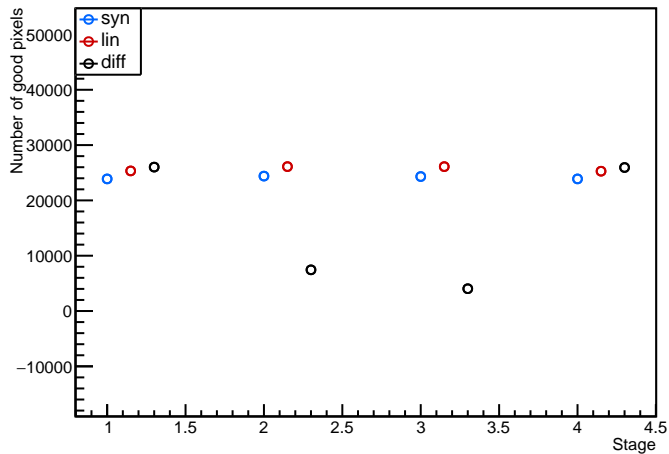
Module: LivThn1, 20UPGFC0009322 (FE3) discbumpscan Evolution plot (98<occupancy<102)
