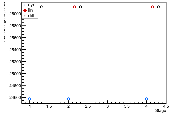
Module: LivThn1, 20UPGFC0009306 (FE2) digitalscan Evolution plot (97<occupancy<103)
