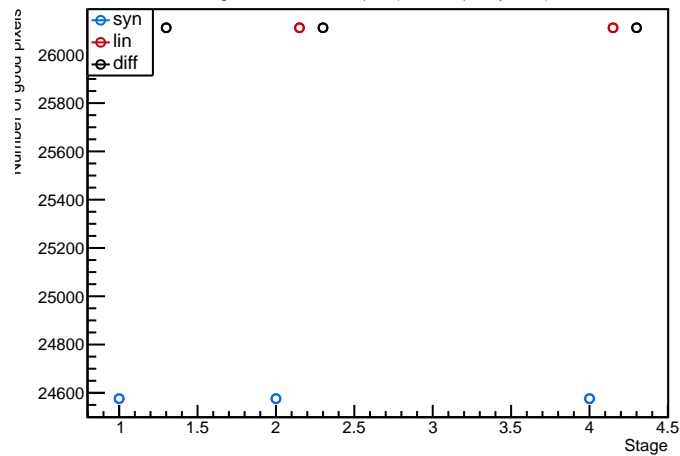
Module: LivThn1, 20UPGFC0009370 (FE4) digitalscan Evolution plot (97<occupancy<103)
