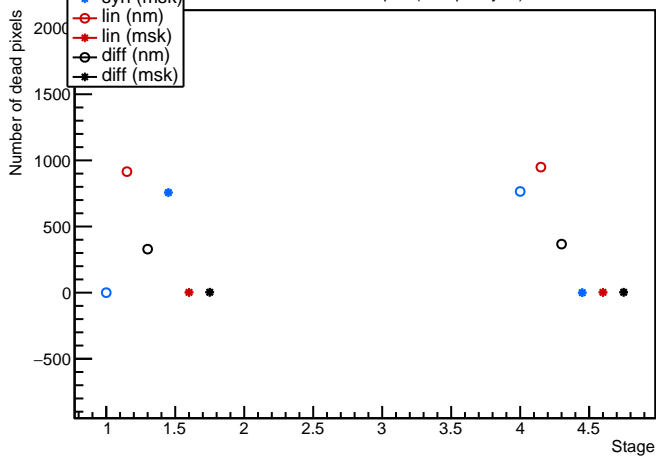
Module: LivThn1, 20UPGFC0009274 (FE1) crosstalkscan Evolution plot (occupancy=0)
