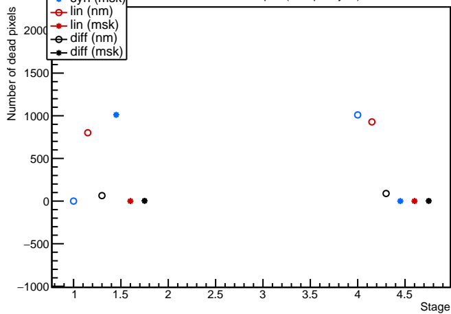
Module: LivThn1, 20UPGFC0009370 (FE4) crosstalkscan Evolution plot (occupancy=0)
