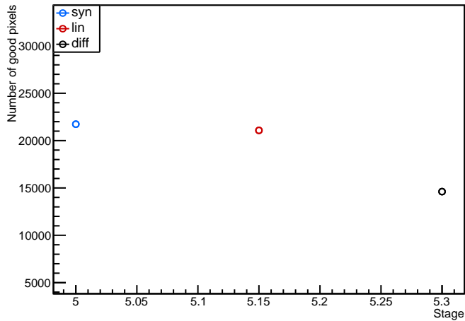
Module: Ox9, A9_Chip3 (FE3) discbumpscan Evolution plot (98<occupancy<102)
