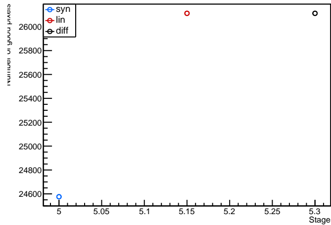
Module: Ox9, A9_Chip2 (FE2) digitalscan Evolution plot (97<occupancy<103)
