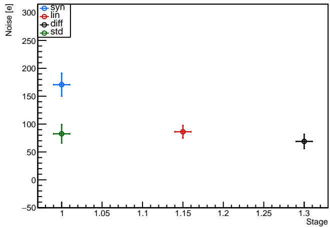
Module: Ox11, A11_Chip3 (FE3) NoiseDist Evolution plot
