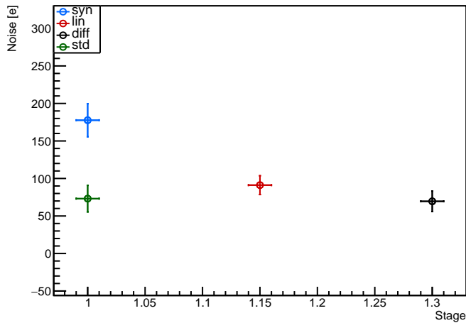
Module: Ox11, A11_Chip1 (FE1) NoiseDist Evolution plot
