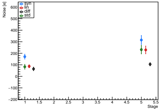
Module: Ox11, A11_Chip4 (FE4) NoiseDist Evolution plot
