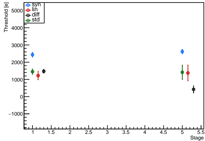
Module: Ox11, A11_Chip4 (FE4) ThresholdDist Evolution plot
