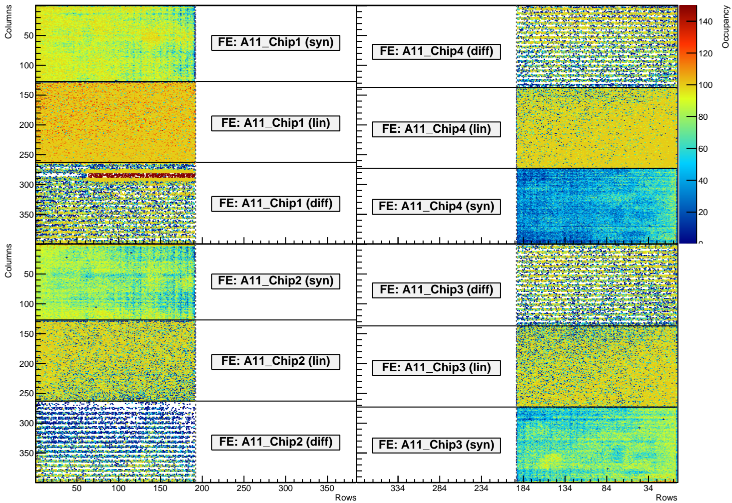
discbumpscan OccupancyMap (Module: Ox11) (Stage1)
