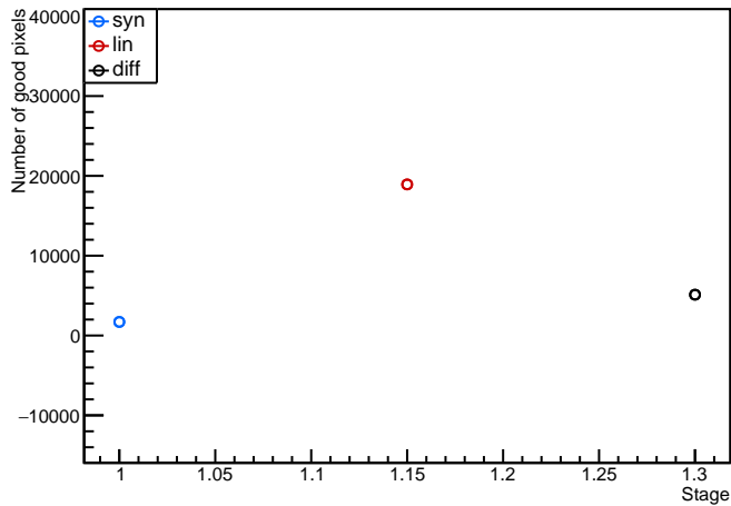
Module: Ox11, A11_Chip1 (FE1) discbumpscan Evolution plot (98<occupancy<102)
