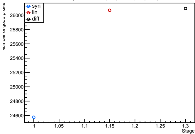
Module: Ox11, A11_Chip2 (FE2) analogscan Evolution plot (97<occupancy<103)
