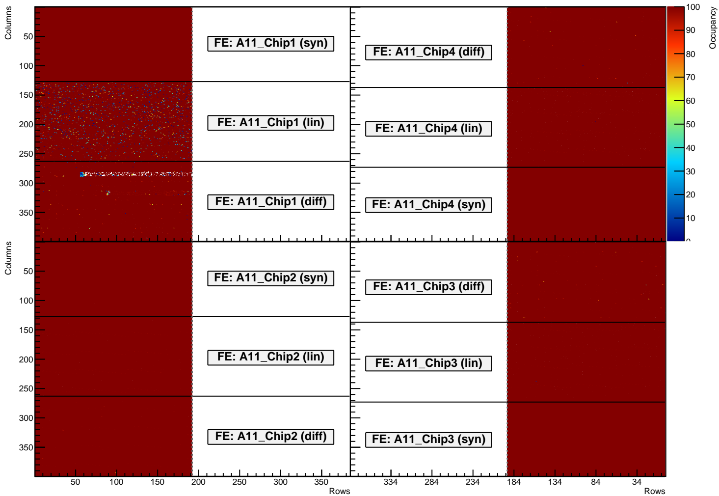
analogscan OccupancyMap (Module: Ox11) (Stage1)
