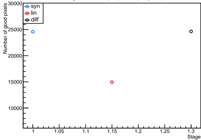
Module: Ox11, A11_Chip1 (FE1) analogscan Evolution plot (97<occupancy<103)
