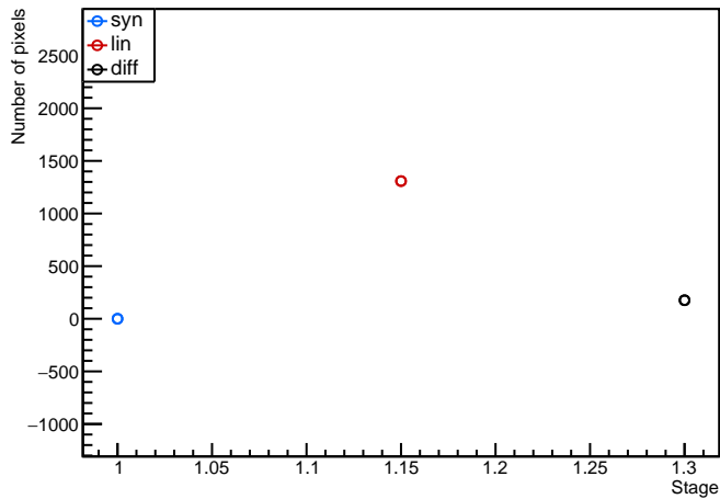
Module: Ox11, A11_Chip1 (FE1) analogscan Evolution plot (0<occupancy<98)
