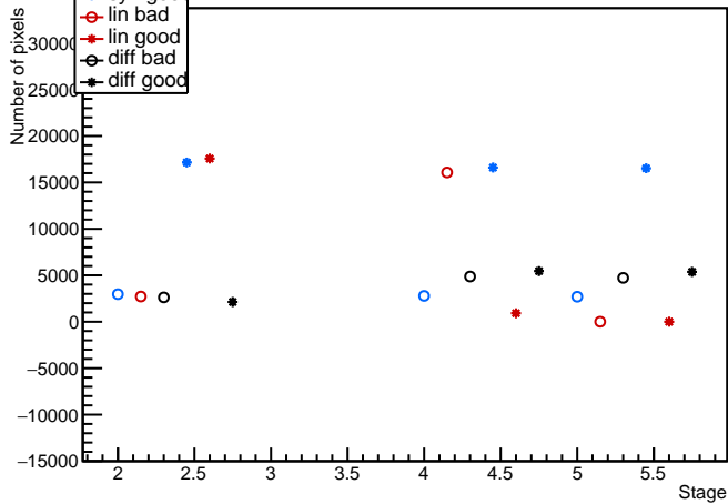
Module: MilanQ2, 20UPGFC0012412 (FE2) discbumpscan Evolution plot (analysis)
