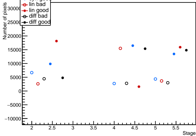
Module: MilanQ2, 20UPGFC0012442 (FE1) discbumpscan Evolution plot (analysis)
