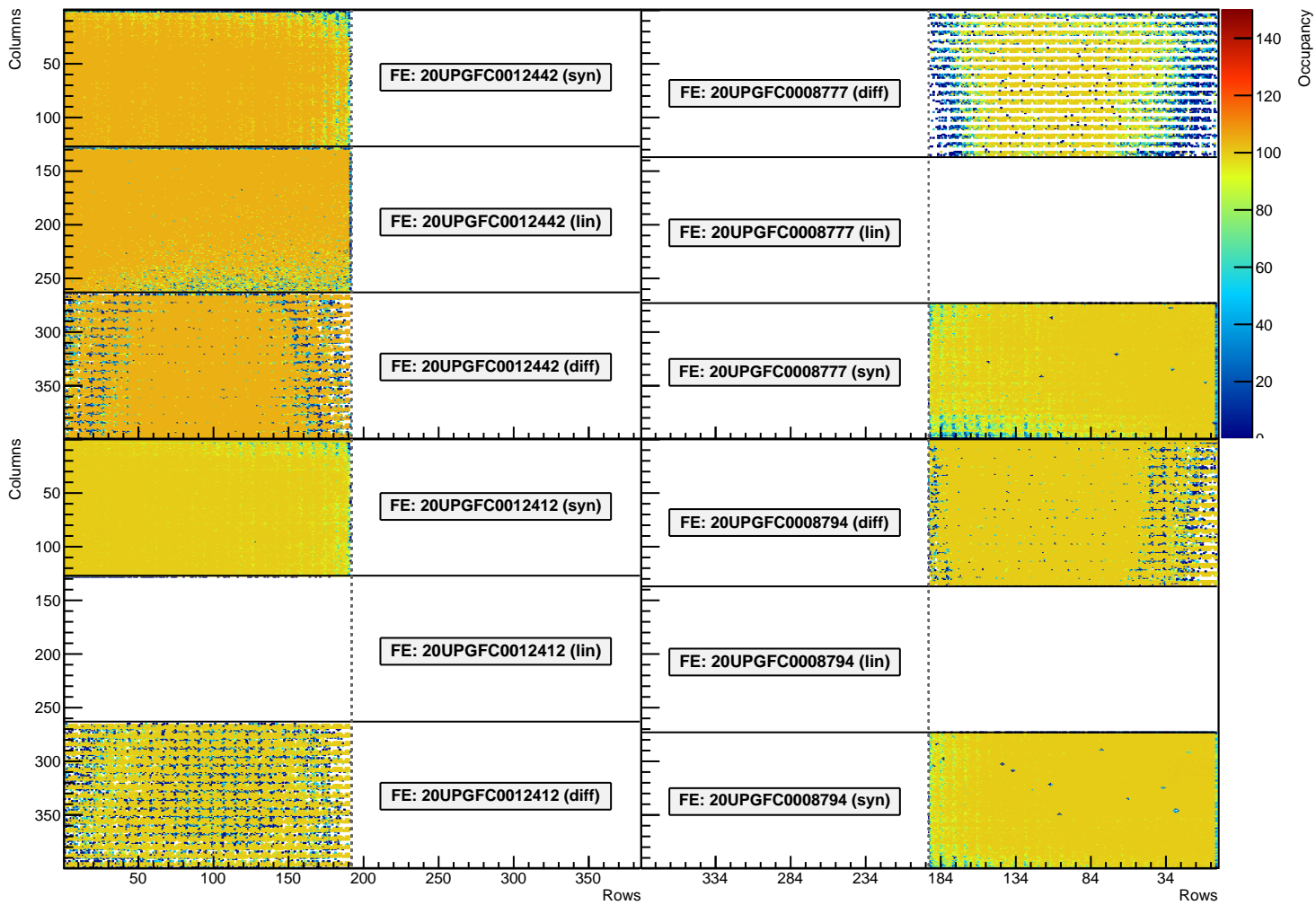
discbumpscan OccupancyMap (Module: MilanQ2) (Stage5)
