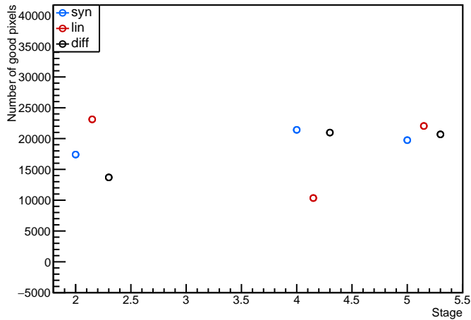
Module: MilanQ2, 20UPGFC0012442 (FE1) discbumpscan Evolution plot (98<occupancy<102)
