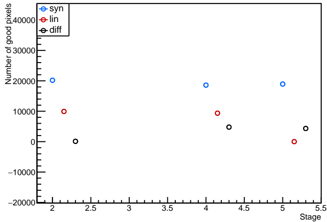
Module: MilanQ2, 20UPGFC0008777 (FE4) discbumpscan Evolution plot (98<occupancy<102)
