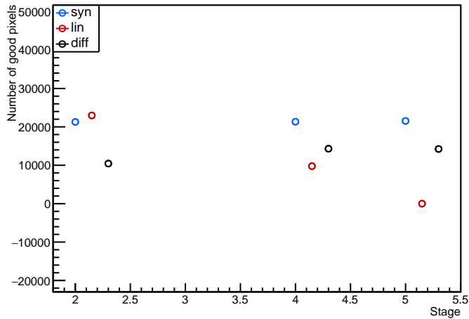
Module: MilanQ2, 20UPGFC0012412 (FE2) discbumpscan Evolution plot (98<occupancy<102)
