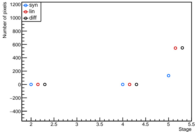
Module: MilanQ2, 20UPGFC0012412 (FE2) digitalscan Evolution plot (0<occupancy<98)
