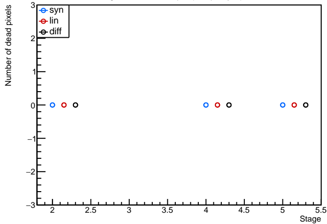
Module: MilanQ2, 20UPGFC0008777 (FE4) digitalscan Evolution plot (occupancy=0)
