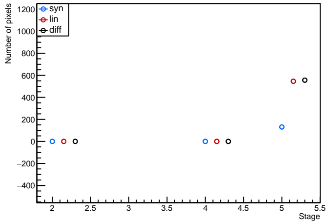
Module: MilanQ2, 20UPGFC0008794 (FE3) digitalscan Evolution plot (0<occupancy<98)
