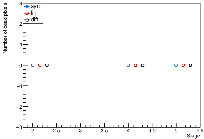
Module: MilanQ2, 20UPGFC0012412 (FE2) digitalscan Evolution plot (occupancy=0)
