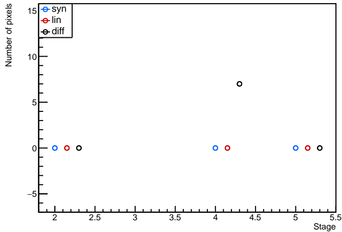
Module: MilanQ2, 20UPGFC0008777 (FE4) analogscan Evolution plot (occupancy>102)
