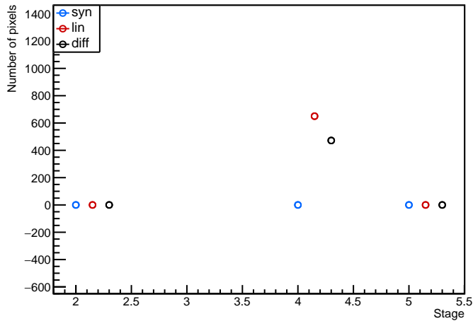
Module: MilanQ2, 20UPGFC0008794 (FE3) analogscan Evolution plot (occupancy>102)
