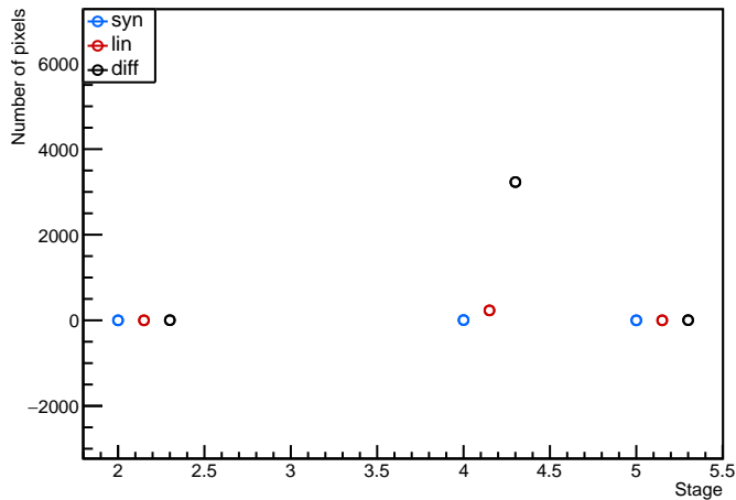
Module: MilanQ2, 20UPGFC0008794 (FE3) analogscan Evolution plot (0<occupancy<98)
