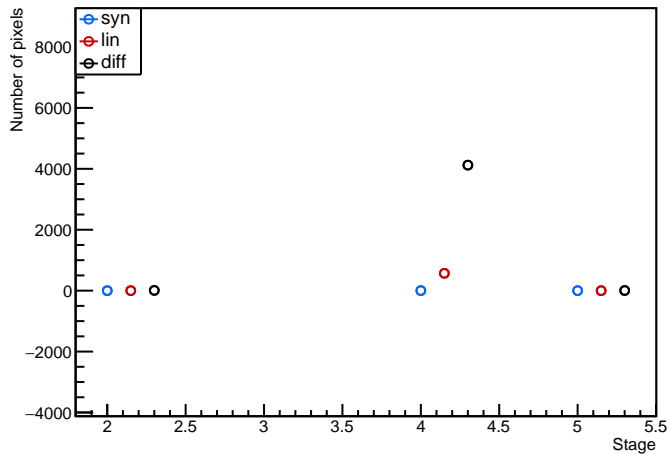
Module: MilanQ2, 20UPGFC0012442 (FE1) analogscan Evolution plot (0<occupancy<98)
