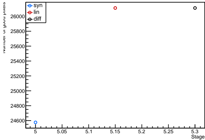
Module: LivThn4, 20UPGFC0009322 (FE3) digitalscan Evolution plot (97<occupancy<103)
