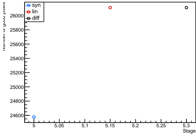
Module: LivThn4, 20UPGFC0009370 (FE4) digitalscan Evolution plot (97<occupancy<103)
