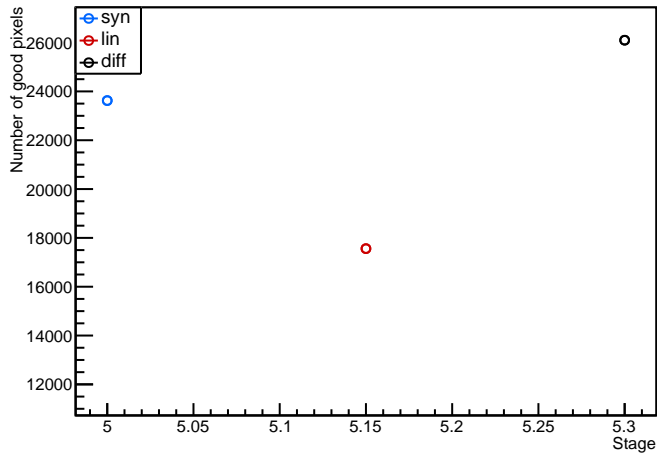
Module: LivThn4, 20UPGFC0009306 (FE2) analogscan Evolution plot (97<occupancy<103)
