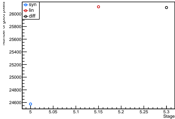
Module: LivThn4, 20UPGFC0009322 (FE3) analogscan Evolution plot (97<occupancy<103)
