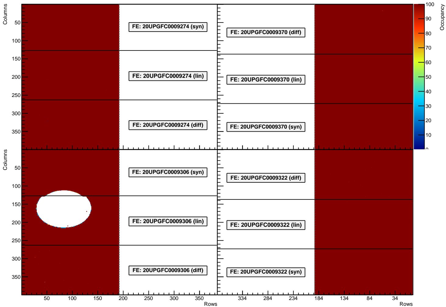
analogscan OccupancyMap (Module: LivThn4) (Stage5)
