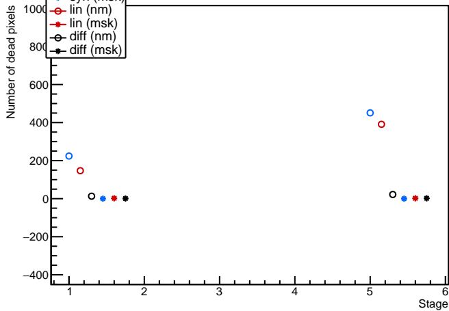
Module: LivThn1, 20UPGFC0009274 (FE1) discbumpscan Evolution plot (occupancy=0)
