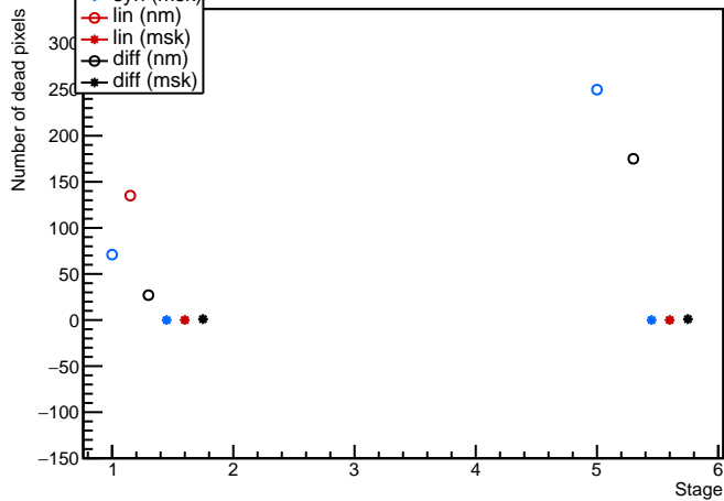
Module: LivThn1, 20UPGFC0009370 (FE4) discbumpscan Evolution plot (occupancy=0)
