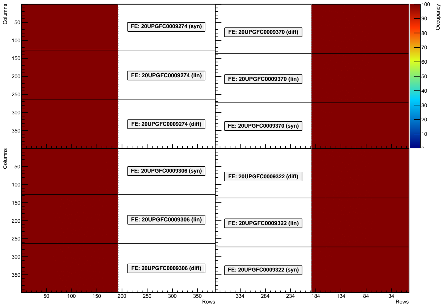
digitalscan OccupancyMap (Module: LivThn1) (Stage5)
