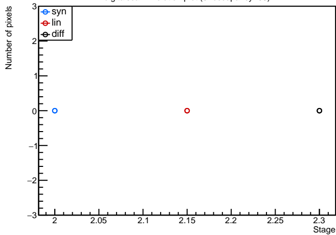
Module: LivThn3, 20UPGFC0009323 (FE4) digitalscan Evolution plot (0<occupancy<98)
