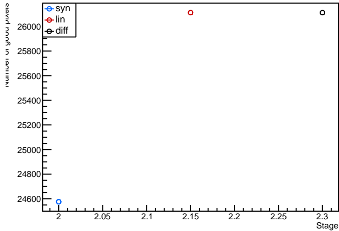
Module: LivThn3, 20UPGFC0009323 (FE4) digitalscan Evolution plot (97<occupancy<103)
