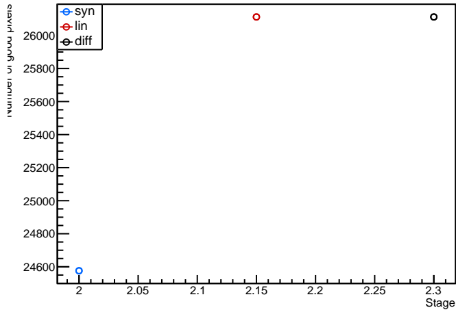
Module: LivThn3, 20UPGFC0009291 (FE1) digitalscan Evolution plot (97<occupancy<103)
