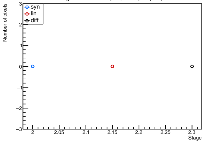
Module: LivThn3, 20UPGFC0009291 (FE1) digitalscan Evolution plot (0<occupancy<98)
