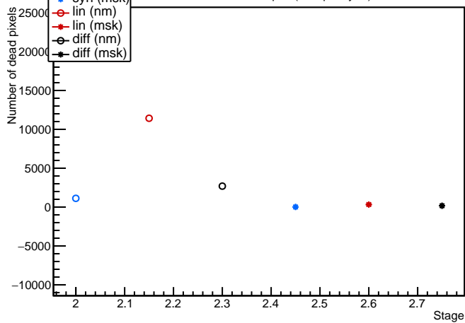
Module: LivThn3, 20UPGFC0009307 (FE3) crosstalkscan Evolution plot (occupancy=0)
