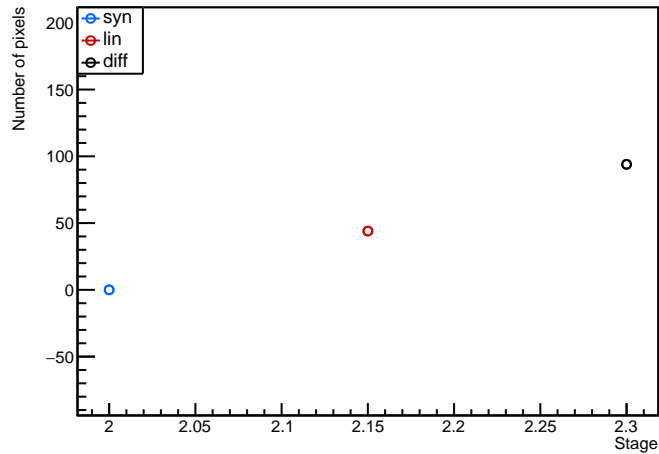
Module: LivThn3, 20UPGFC0009307 (FE3) analogscan Evolution plot (0<occupancy<98)
