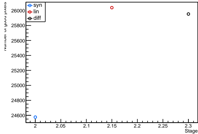
Module: LivThn3, 20UPGFC0009292 (FE2) analogscan Evolution plot (97<occupancy<103)
