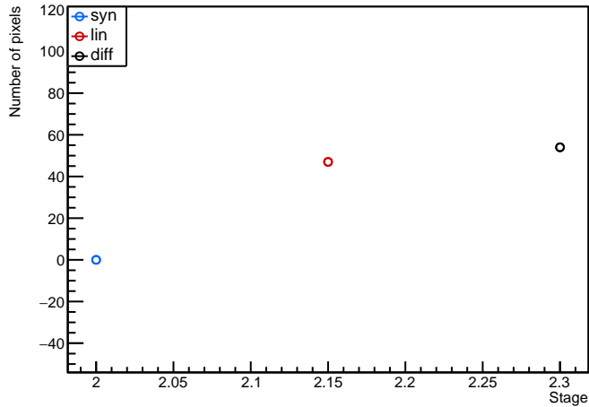
Module: LivThn3, 20UPGFC0009292 (FE2) analogscan Evolution plot (occupancy>102)
