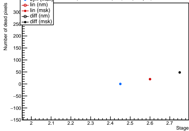
Module: LivThn2, 20UPGFC0009369 (FE3) discbumpscan Evolution plot (occupancy=0)
