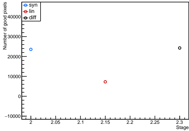
Module: LivThn2, 20UPGFC0009337 (FE1) discbumpscan Evolution plot (98<occupancy<102)
