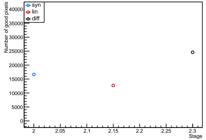
Module: LivThn2, 20UPGFC0009369 (FE3) discbumpscan Evolution plot (98<occupancy<102)
