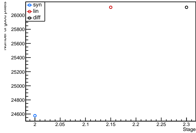
Module: LivThn2, 20UPGFC0009353 (FE2) digitalscan Evolution plot (97<occupancy<103)
