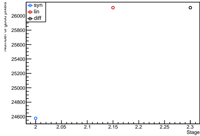
Module: LivThn2, 20UPGFC0009337 (FE1) digitalscan Evolution plot (97<occupancy<103)
