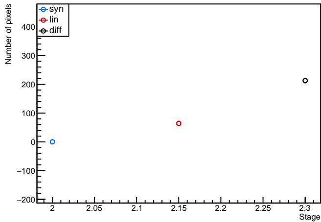
Module: LivThn2, 20UPGFC0009337 (FE1) analogscan Evolution plot (0<occupancy<98)
