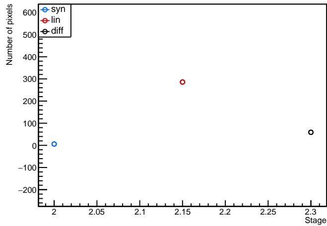
Module: LivThn2, 20UPGFC0009369 (FE3) analogscan Evolution plot (occupancy>102)
