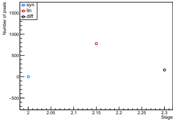
Module: LivThn2, 20UPGFC0009353 (FE2) analogscan Evolution plot (0<occupancy<98)
