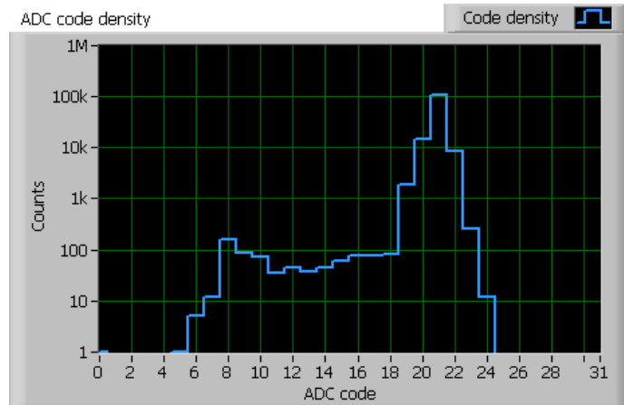
Figure 20 Spectrum of X-rays from an ^{55}\text{Fe} source recorded using a CPC2 sensor with CPD1 drive and CPR2 readout chips, demonstrating for the first time the operation of all the elements needed for the production of a CCD ladder.
