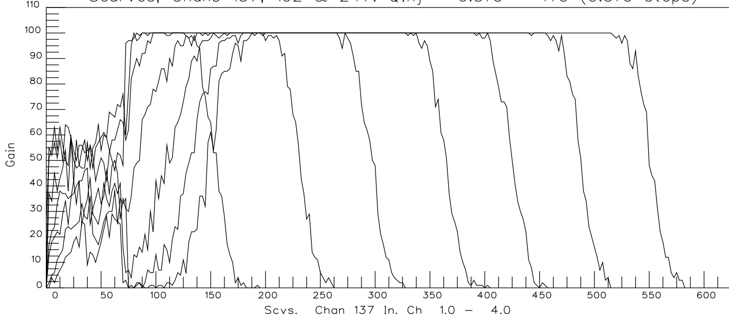
Scurves, Chans 137, 192 & 247. Q_{inj} = 0.5fC - 4fC (0.5fC steps)
