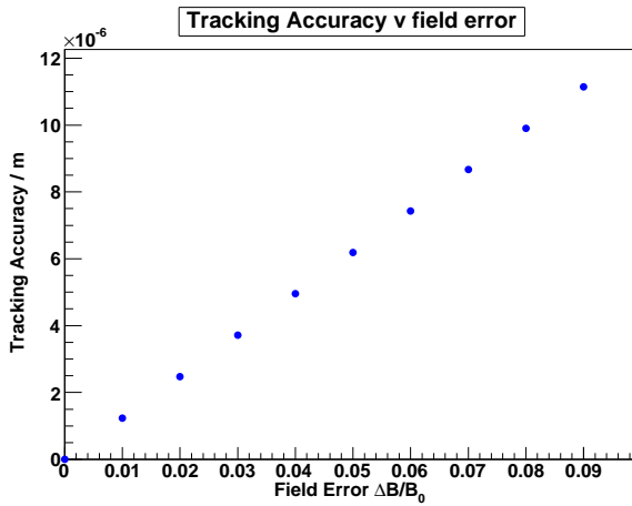
Figure 5: The effect of introducing field errors on the accuracy achieved (compared to an ideal trajectory) when tracking an electron through 155 periods of an undulator.
