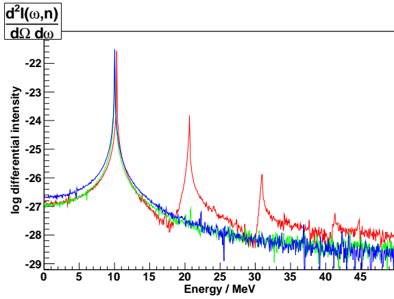
Figure 2: The energy spectra calculated when tracking an electron through a 1255 period undulator. In each case the radiation was calculated at 10 points per period, although the particle tracking was performed using 10 (red), 100 (green) and 1000 (blue) steps per period. Note that by using Lie maps, each of the 3 calculations took the same amount of time despite the increase in tracking accuracy.
