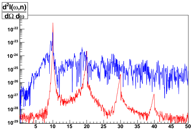
Figure 6: Introducing field errors to the undulator field causes a deterioration of the calculated energy spectrum of synchrotron radiation. Field errors of magnitude \Delta B/B_0 = 0.001 (red) and 0.01 (blue) were used in these calculations c.f. the green points in figure 3 for comparison with the spectrum calculated with no field errors.
