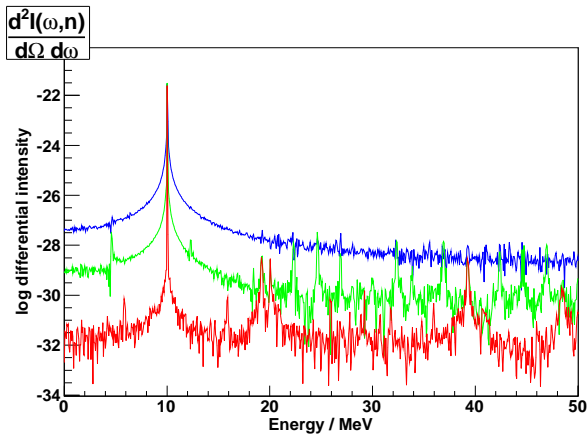
Figure 3: The energy spectra observed from an electron passing through a 155 period undulator. The emitted radiation was calculated at a rate of 10 (blue), 100 (green) and 1000 (red) steps per period.
