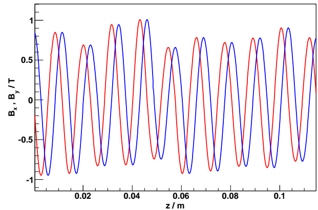
Figure 4: The magnetic field B_x (red) and B_y (blue) in a section of a helical undulator. Field errors which vary every half period are included in the field description. In this case \Delta B/B_0 = 0.10 is used for illustration only
