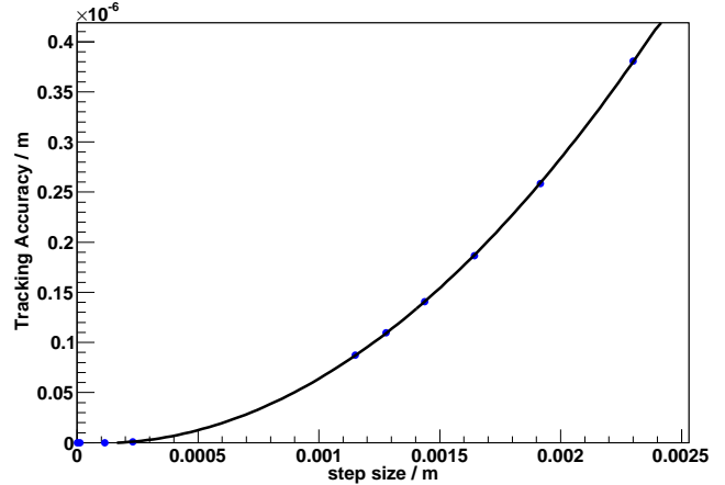
Figure 1: Tracking an electron through a 155 period undulator. The electrons deviation from an analytic trajectory at the undulator exit is plotted as a function of the step size used to integrate the equations of motion.
