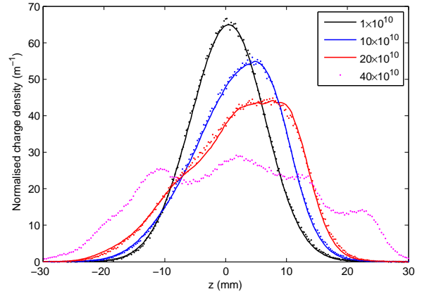
Figure 7: Variation of longitudinal charge distribution with bunch population in presence of wake files generated by all BPM insertions and absorbers. Points represent the results of a tracking simulation, lines show the solution of the Haissinski equation. Arc cell phase advance is 100^\circ .
