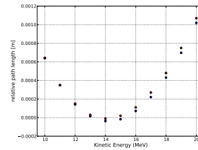
Figure 2: Path length versus kinetic energy from dynamical map (blue) and PyZgoubi (red).
