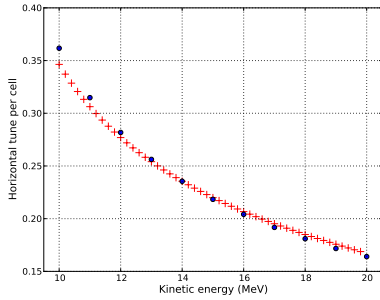
Figure 4: Horizontal betatron tunes computed with a set of dynamical maps at different reference energies (blue dots), and with a single dynamical map with different energy deviations (red crosses).
