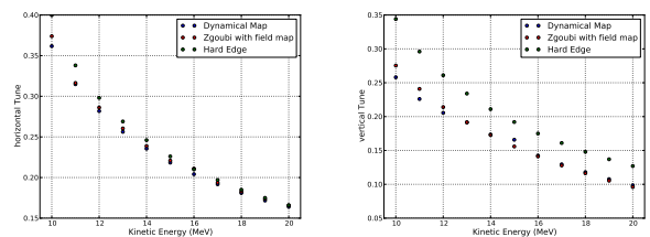
Figure 3: Betatron motion with multiple dynamical maps.
