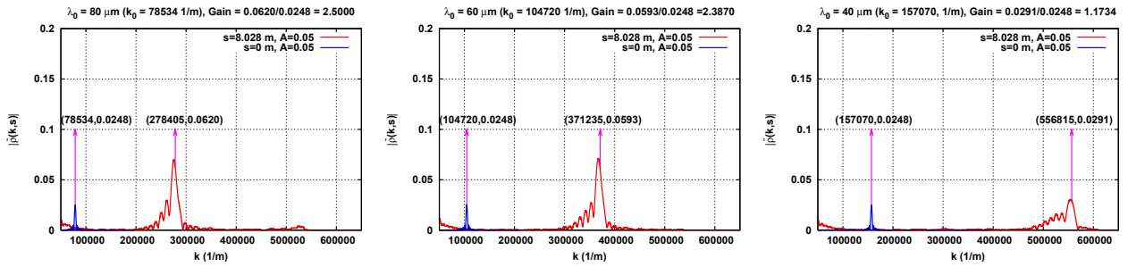
Figure 3: Spectra at s = 0 and s = s_f , for \lambda_0 = 80\mu\text{m} (left) and \lambda_0 = 60\mu\text{m} (center) and \lambda_0 = 40\mu\text{m} (right).
