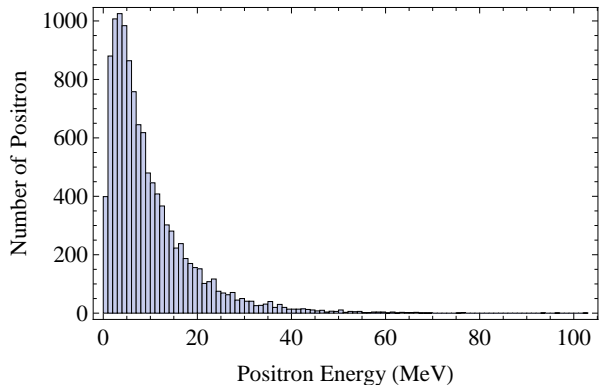
Figure 2: Positron energy spread immediately after the target, for undulator parameters Option 1.
