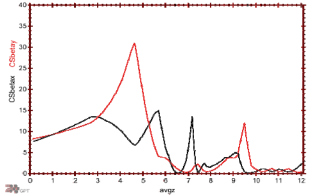
Figure 5: \beta_{x,y} for the tomography section of the ALICE to EMMA injection line from GPT at 35 MeV and 0 pC. (Note that zero metres on this and subsequent plots correspond to s = 15.7 m on the MAD results)
