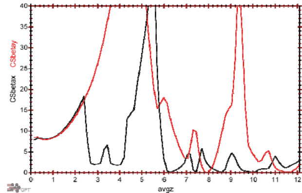
Figure 6: \beta_{x,y} for the tomography section of the ALICE to EMMA injection line from GPT at 35 MeV and 80 pC, with no correction for space charge.
