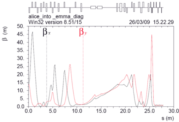
Figure 3: \beta_{x,y} for the ALICE to EMMA injection line.
