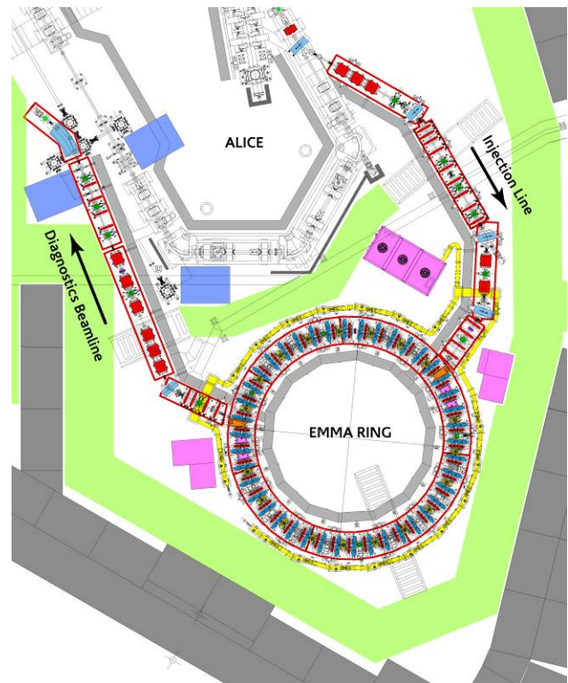
Figure 1: Layout of ALICE & EMMA.
