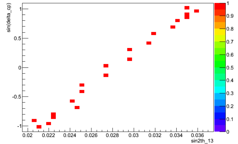
\sin(\delta_{cp}): \sin^2\theta_{13}
