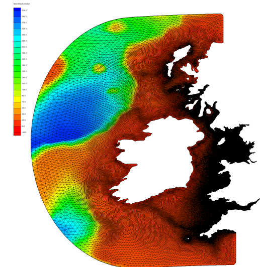
2-D modelling of tidal hydrodynamics
