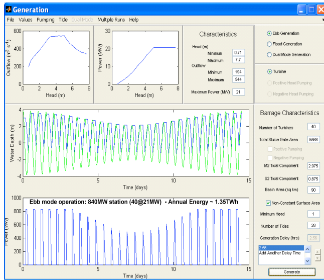
0-D modelling of energy generation
