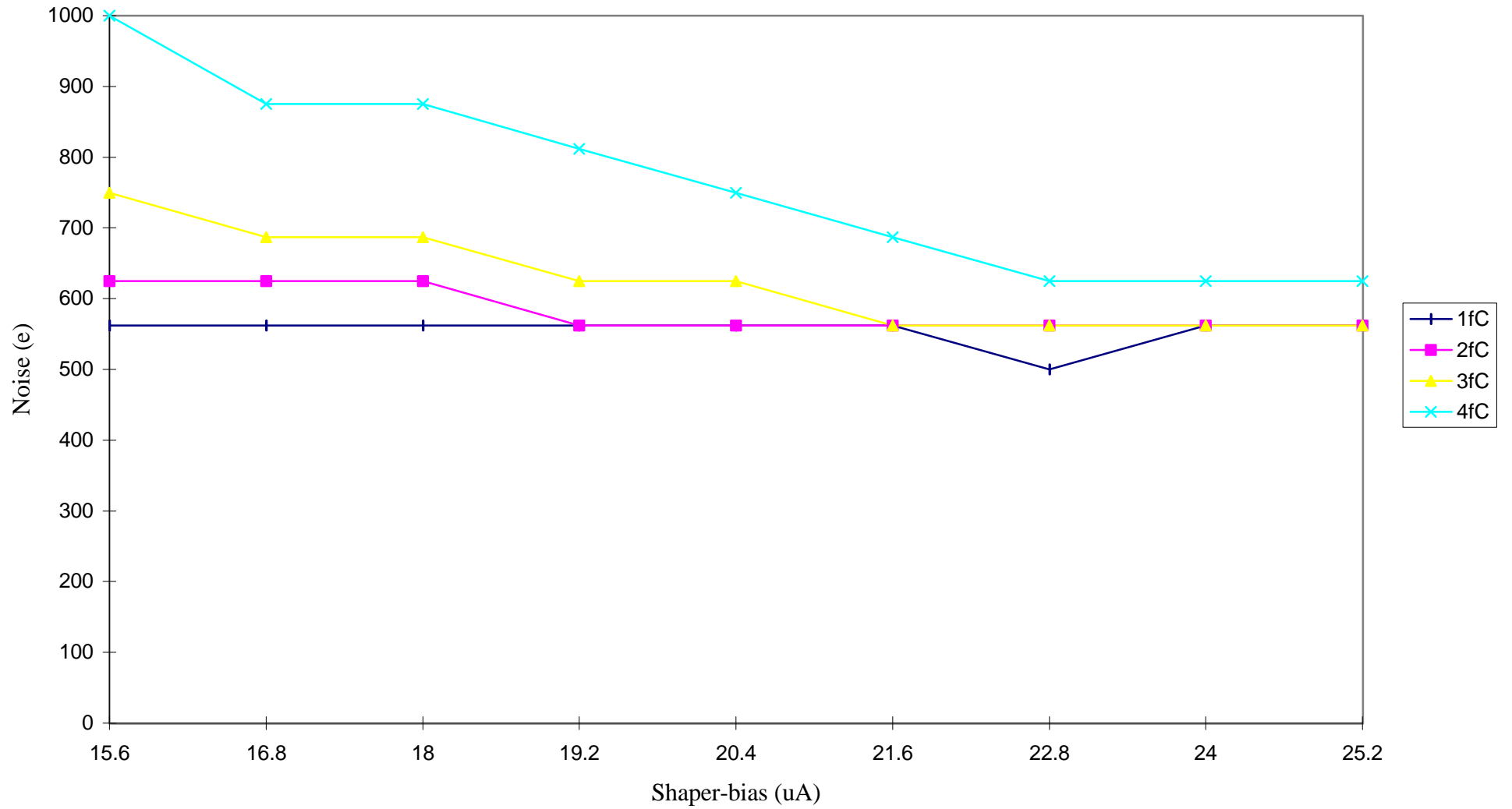
ABCD2 (Thinned) Master Chip only Input Noise as a function of Shaper-bias for 1fC - 4fC calibration
