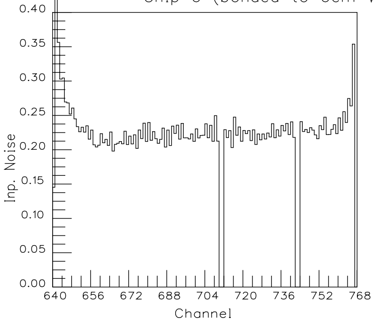
Chip 6 (bonded to 6cm Wedge detector) Vcal = 3.0fC
